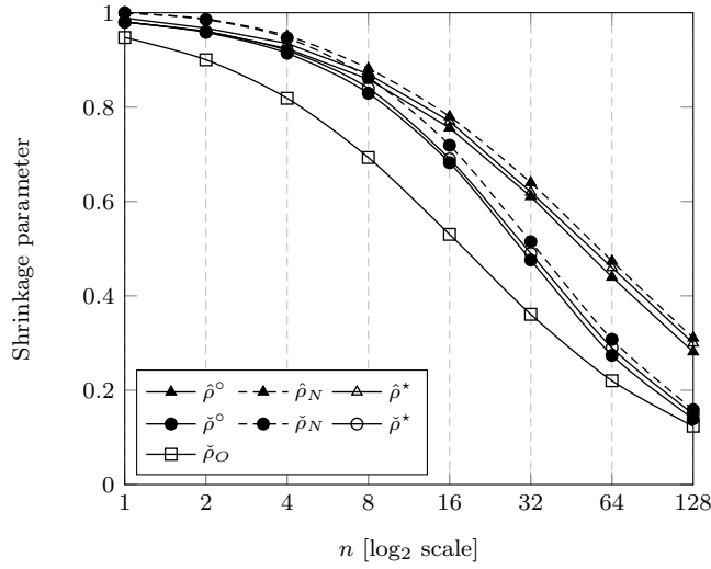
Figure 5: Shrinkage parameter \rho averaged over 10 000 Monte Carlo simulations, for N = 32 , various values of n , [C_N]_{ij} = r^{|i-j|} with r = 0.7 ; \hat{\rho}_N and \check{\rho}_N given in Proposition 2; \check{\rho}_O is the clairvoyant estimator proposed in (Chen et al., 2011, Equation (12)); \rho^* , \hat{\rho}^* , and \check{\rho}^* taken with c = N/n ; \hat{\rho}^o = \operatorname{argmin}_{\{\rho \in (\max\{0, 1-c_N^{-1}\}, 1]\}} \{\hat{D}_N(\rho)\} and \check{\rho}^o = \operatorname{argmin}_{\{\rho \in (0, 1]\}} \{\check{D}_N(\rho)\} .
